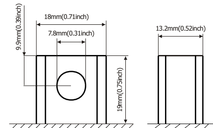
Terminal Dimensions
